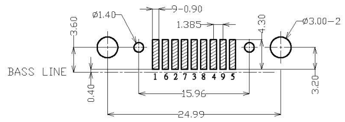
P.C.B. LAYOUT(TOLERANCE±0.05) TOP VIEW
