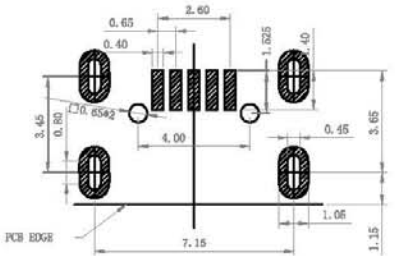
RECOMMENDED PCB LAYOUT (TOL: ±0.05)
