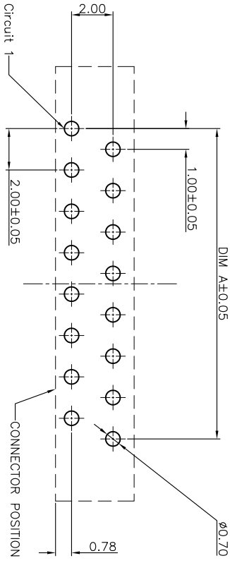
RECOMMENDED PCB PATTERN LAYOUT
