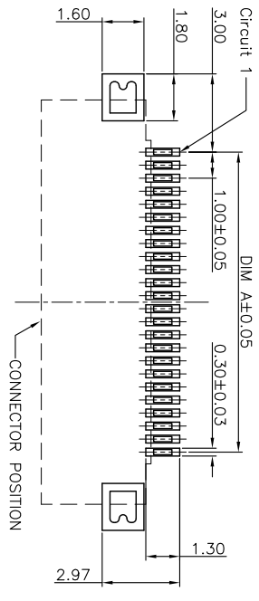
RECOMMENDED PCB PATTERN LAYOUT
