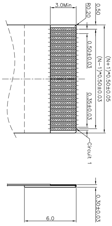
RECOMMENDED FPC/FPC DIMENSION
