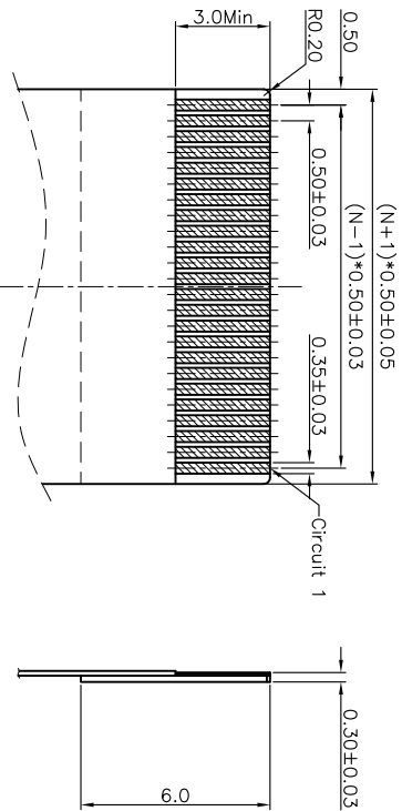
RECOMMENDED PFC/FCC DIMENSION
