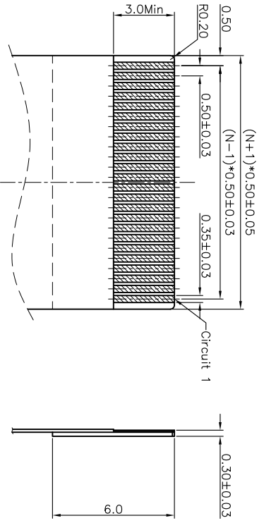
RECOMMENDED P.C.B. PATTERN LAYOUT
