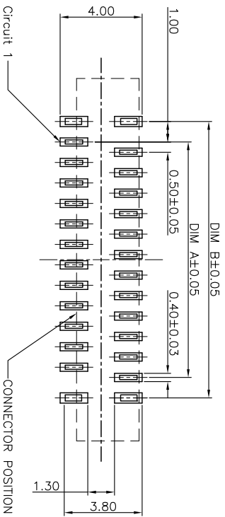
RECOMMENDED P.C.B. PATTERN LAYOUT
