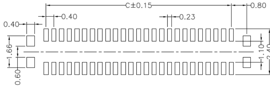
RECOMMENDED PCB LAYOUT CONNECTOR SIDE
